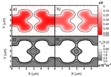
Fig. 1. (a) and (c) considers only the gated sample, whereas b) and d) is for both etched and trench gated structure. a) and b) simulate the potential profiles of the sample and the corresponding electron densities are shown in (c) and (d). We set the same gate voltage (-1.8 V, note that surface potential is -0.7 V due to mid-gap pinning) for both situations. Potential distribution of the gated sample presents smooth characteristic, however, the potential profile of the trench gated structure is very sharp. Hence the electron density at the island center is higher in (d) compared to (c), in the island center. All the figures are obtained at zero temperature and magnetic field.
