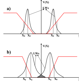
Fig. 3. The (screened) potential and the shift of the LWs for different magnetic fields. Slope of the potential is small at higher magnetic field (a) compared to low B value.
